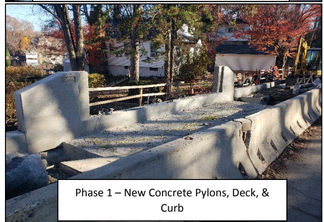
Phase 1 – Concrete Pouring for New Half Bridge Deck Beams & Curb
