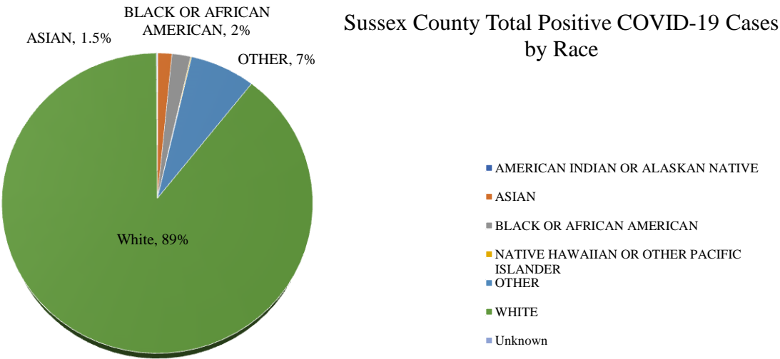
Figure 4: Sussex County Positive COVID-19 Cases by Race
