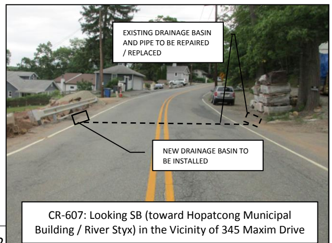
Installation of Drainage System at 345 Maxim Drive to be connected to Roadway Drainage System
